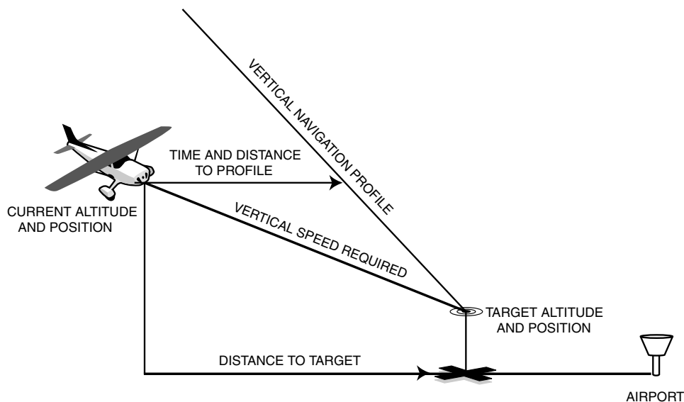
Figure 11-1 VNAV Profile
